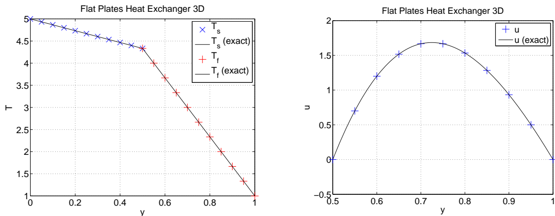
Fig. 13. Results for the 3D flat-plate heat exchanger. The temperature is a piecewise linear profile and the fluid velocity is a cubic polynomial. The numerical solution computed on a Cartesian grid gives the exact solution up to round-off.
