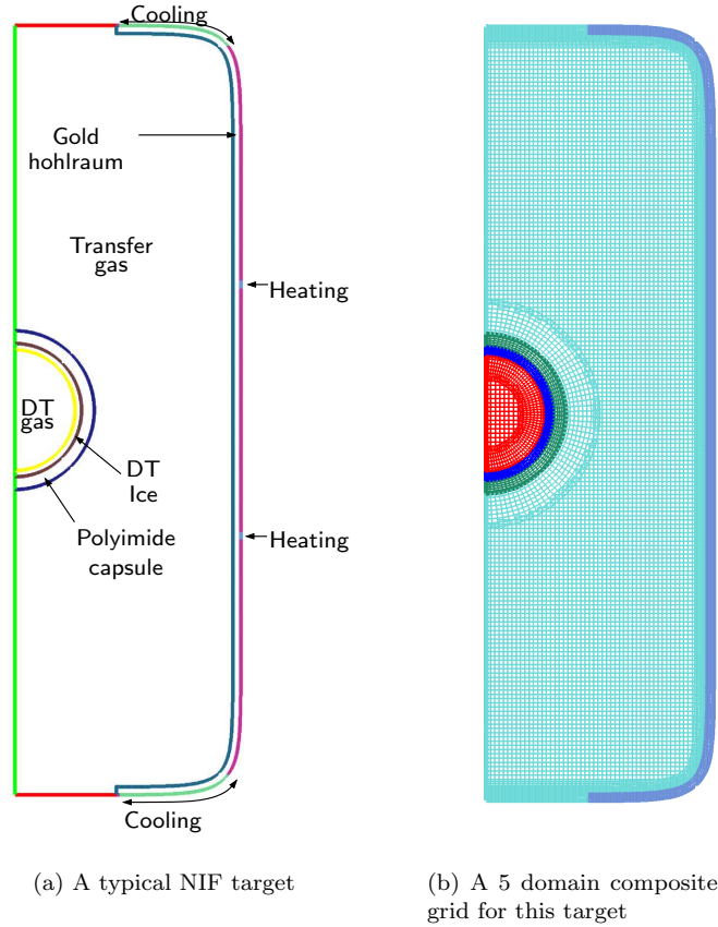
Fig. 25. A typical NIF hohlraum target consists of DT vapor and ice; a polyimide capsule; the heat transfer gas; and the gold hohlraum. The composite grid consists of two fluid and three solid domains using a total of 20 grids.
