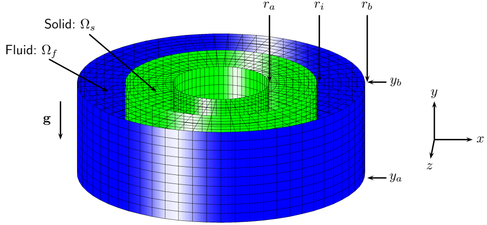
Fig. 15. Cocentric cylinders heat exchanger geometry and grids. The coarse grid \mathcal{G}^{(1)} is shown.
