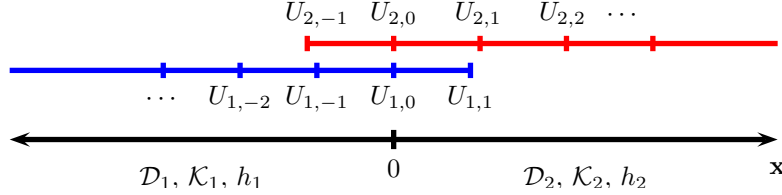
Fig. 6. The overlapping grids for a one-dimensional material interface located at x = 0 . The ghost points U_{2,-1} and U_{1,1} are introduced on the two grids at the interface.
