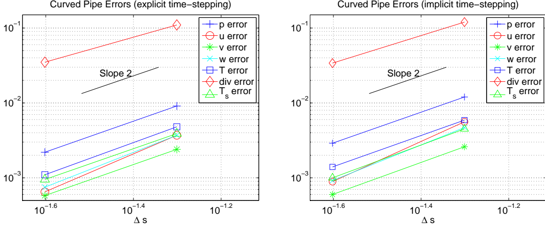
Fig. 21. Maximum errors at t = 1 when solving the fluid in a curved pipe problem using explicit time-stepping and the coupled interface (CI) approach (left) and using implicit time-stepping and the segregated interface (SI) approach (right). See also Figs. 19 and 20.
