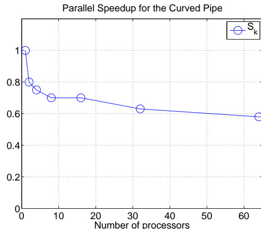
Fig. 24. Parallel speedup, S_k , for the curved pipe. See also Fig. 23.
