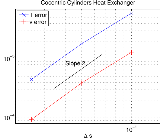
Fig. 17. Maximum errors and estimated convergence rate for the numerical solution of the steady state cocentric cylinders heat exchanger.
