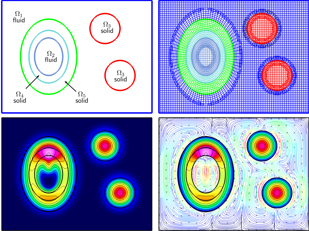
Fig. 1. Top left : a domain \Omega with two fluid sub-domains \Omega_1, \Omega_2 and three solid sub-domains \Omega_3, \Omega_4 and \Omega_5 . Top right: the composite \mathcal{G} consists of five overlapping grids, one for each domain. Bottom left: a computed conjugate heat transfer solution showing the temperature. Bottom right: the streamlines in the fluid domains and the temperature in the solid domains.
