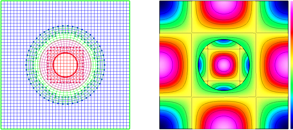
Fig. 8. Left : composite grid \mathcal{G}^{(1)} for the two-domain conjugate heat-transfer problem. The heat equation is solved in the inner disk and the incompressible Navier-Stokes equations are solved in the outer region. Right : the computed temperature for a problem where the exact solution was constructed using the method of analytic solutions.
