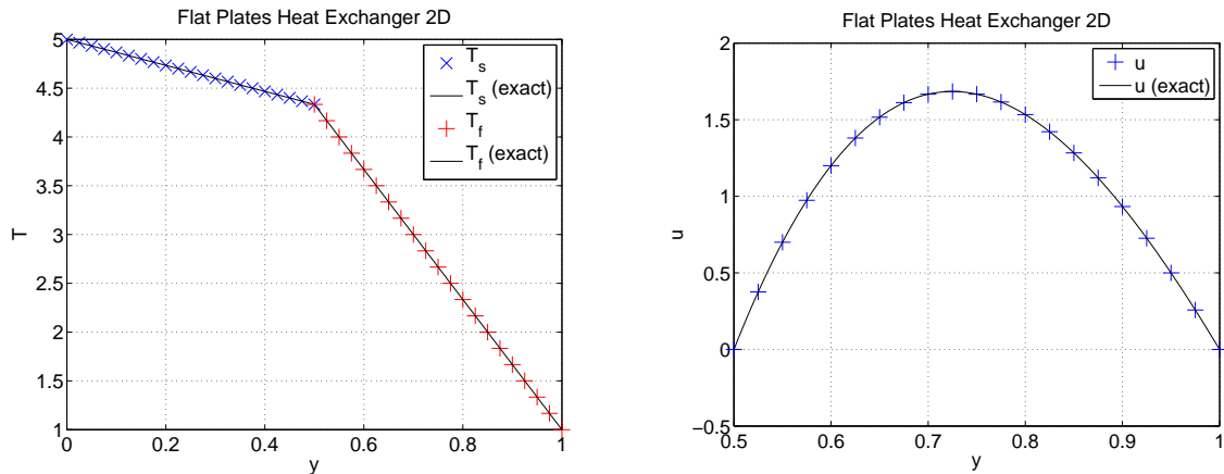
Fig. 12. Results for the 2D flat-plate heat exchanger. The temperature is a piecewise linear profile and the fluid velocity is a cubic polynomial. The numerical solution computed on a Cartesian grid gives the exact solution up to round-off.
