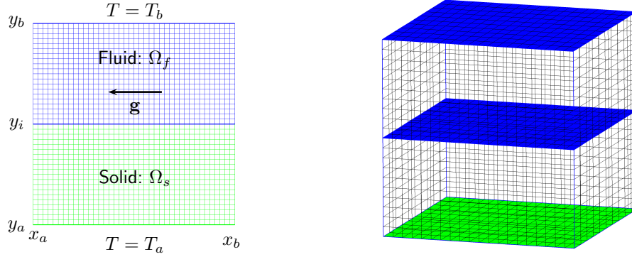
Fig. 11. Flat-plate heat exchanger geometry and grids for the two-dimensional and three-dimensional computations. A rectangular fluid domain sits above a rectangular solid domain.
