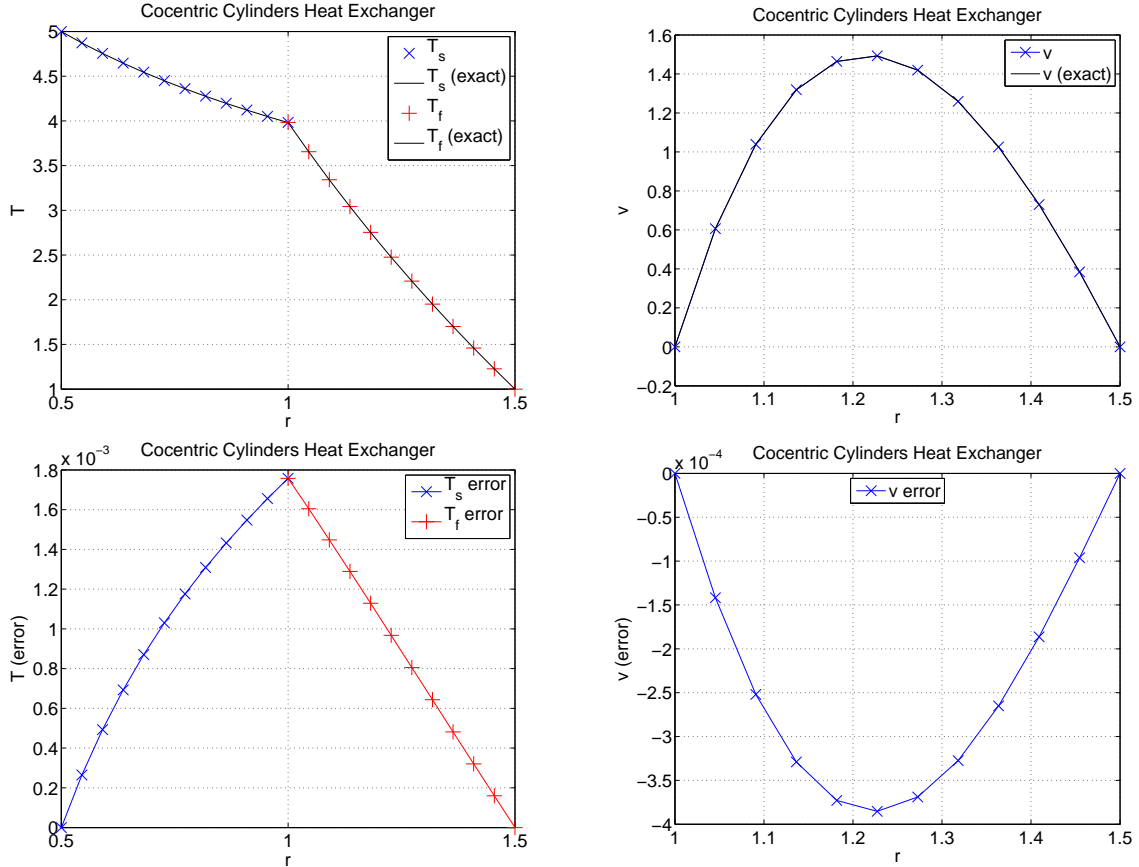
Fig. 16. Results for the cocentric cylinder heat exchanger for grid \mathcal{G}^{(2)} . Left: the computed solution, exact solution and errors for the temperature in the solid and fluid domains along a radial line. Right: the computed solution, exact solution and errors for the velocity component v along a radial line.
