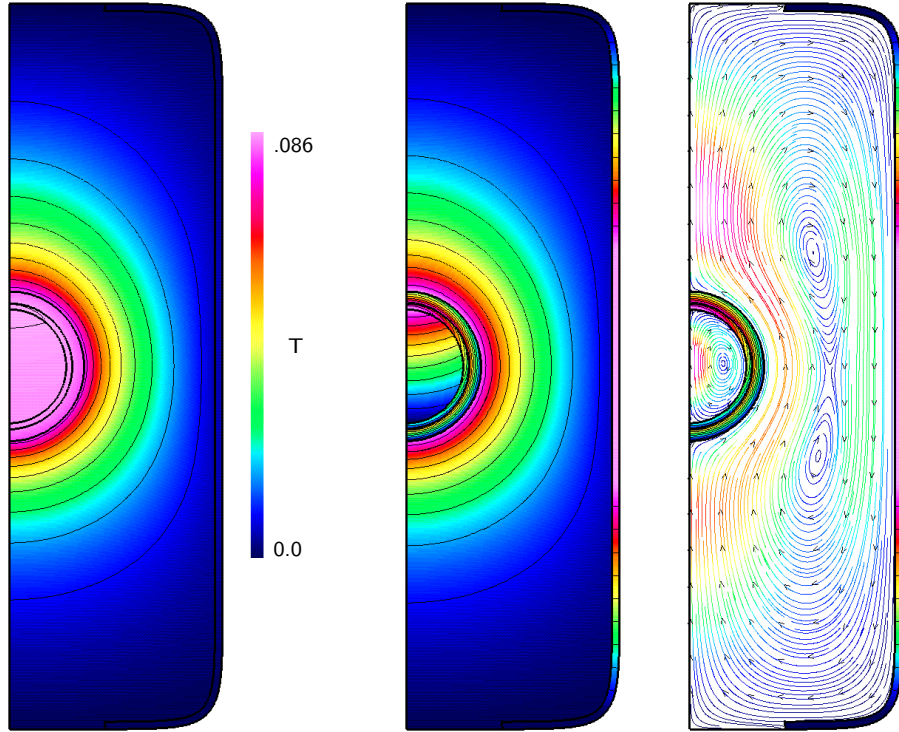
Fig. 27. Hohlräum results. Left: the temperature in each of the domains shown on the same scale. Middle: the temperature is shown with different scales in each domain to better show the variation. For the middle plot the DT vapor has bounds on T of [\.085, \.086] , the DT ice [\.084, \.086] , the capsule [\.081, \.086] , the transfer gas [0., \.083] and hohlräum [0., \.005] . Right: the stream lines in the central DT gas region and transfer gas region. The flow speed in DT vapor has bounds of [0., 1.7 \times 10^{-4}] while the bounds in the transfer gas are [0., \.81] .
